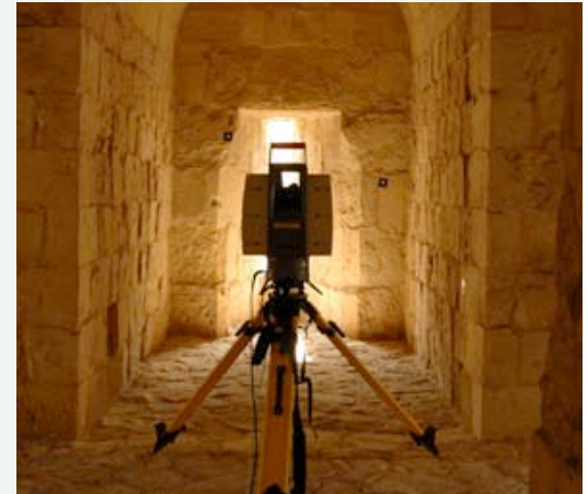
Leica 3D scanner inside the Bab al-Barqiyya, Al-Azhar Park, Cairo, Egypt
